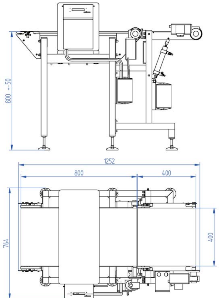
LC 0800x0400 PU with Drop End reject
